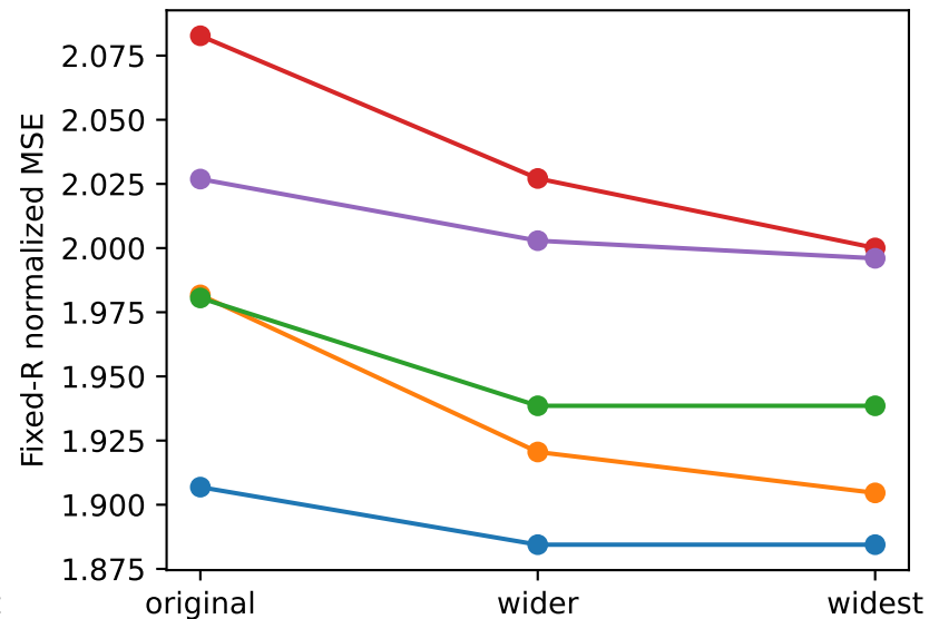
Held-out one-step prediction
