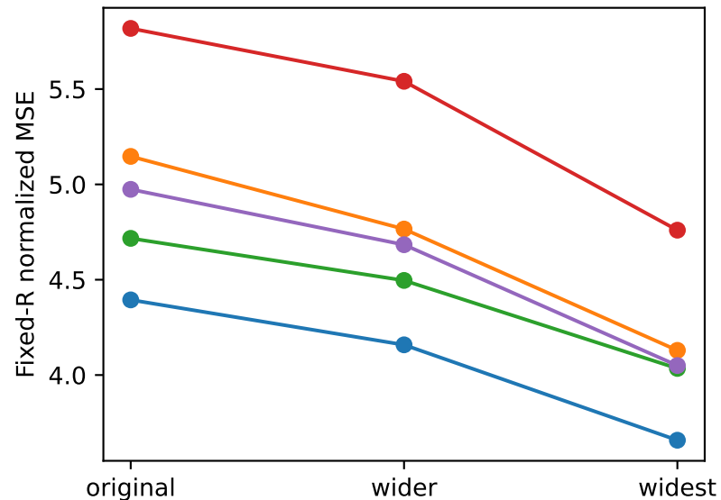
Held-out one-step prediction
