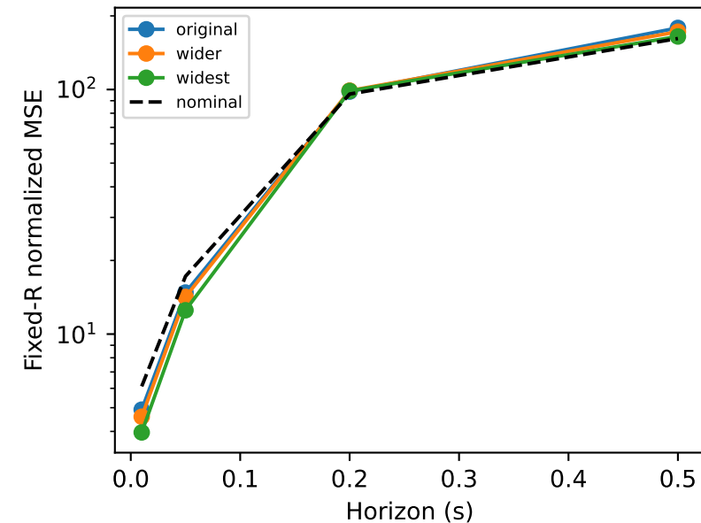
Common-origin held-out forecasts
