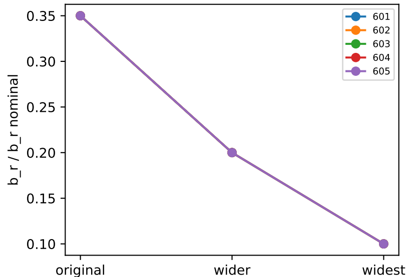
Q scale 0.01: rear gain
