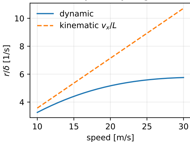
Steady-state yaw gain
