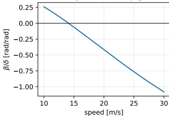
Steady-state sideslip gain
