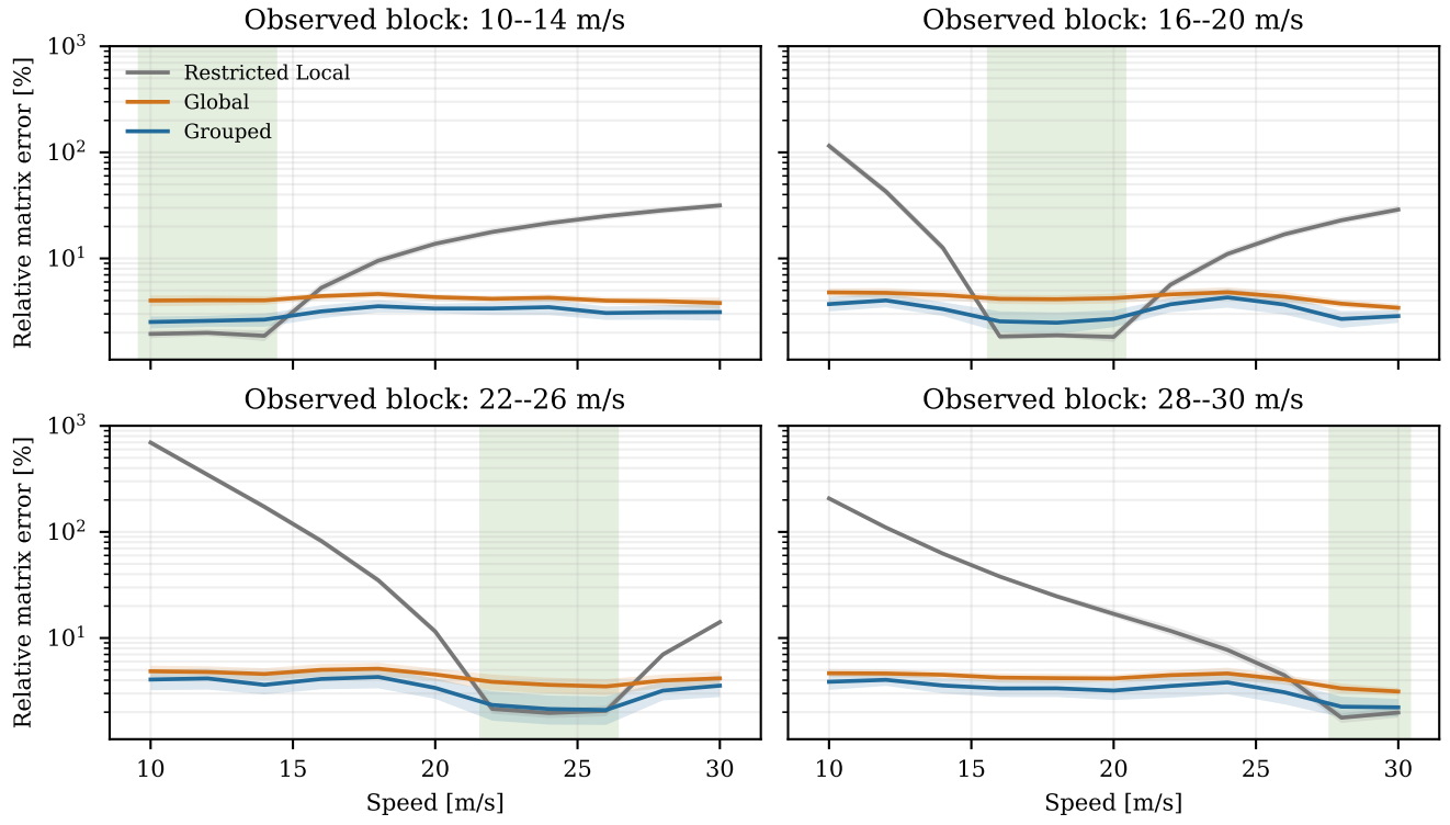
Fig. 1. Label-free matrix error by local coverage block. Shading marks observed speeds. Curves average within block and fleet, then across ten fleets, with pointwise 95% fleet-bootstrap bands. The logarithmic vertical axis retains both Local extrapolation failure and the smaller Global-grouped difference. The curves summarize the primary records; they are not a separate confirmation experiment.
