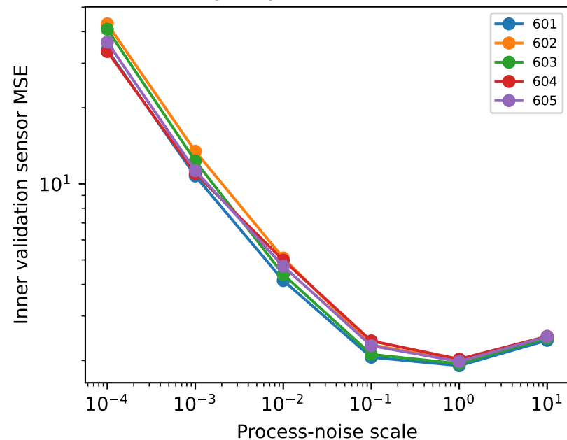
Training-only covariance selection
