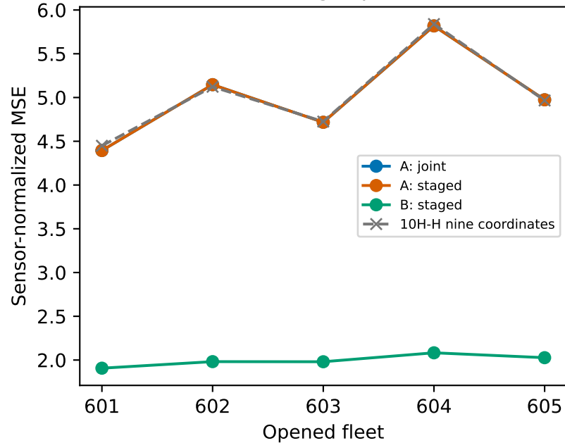
Held-out fixed-weight prediction error
