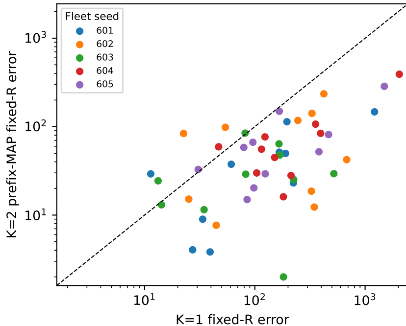
Q scale 1: 50 held-out clients
