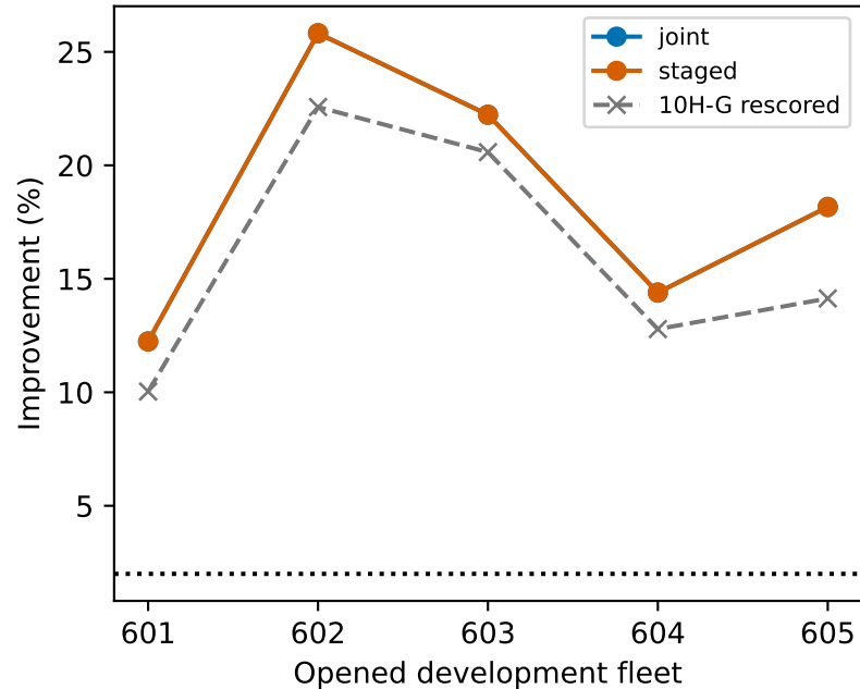
Corrected held-out likelihood
