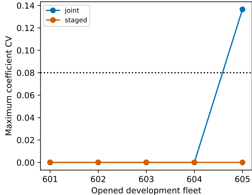
Restart coordinate dispersion
