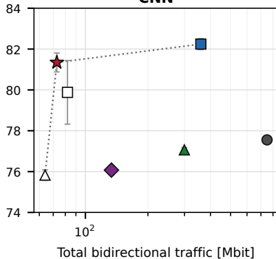
Fashion-MNIST CNN
