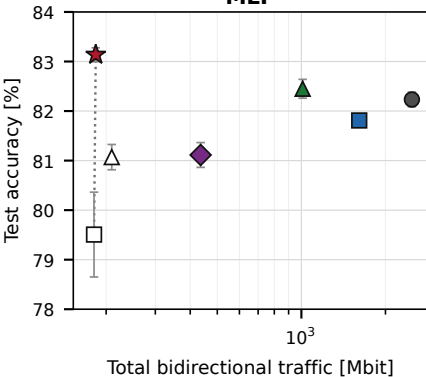
Fashion-MNIST MLP
