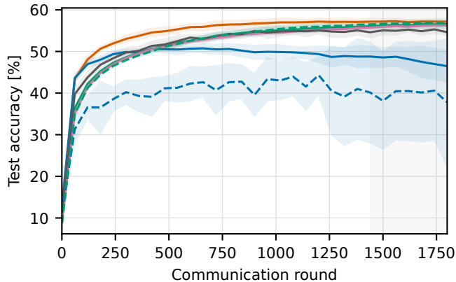
Held-out accuracy
