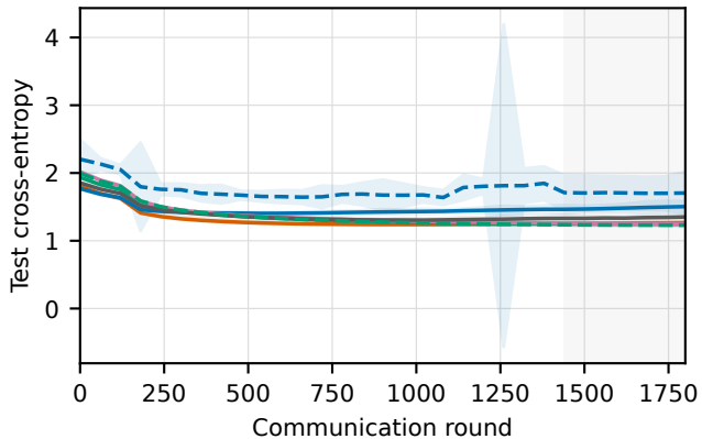
Held-out loss
