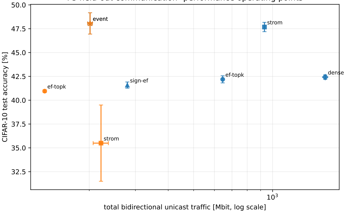
P3 held-out communication--performance operating points
