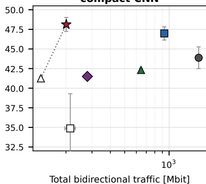
CIFAR-10 compact CNN
