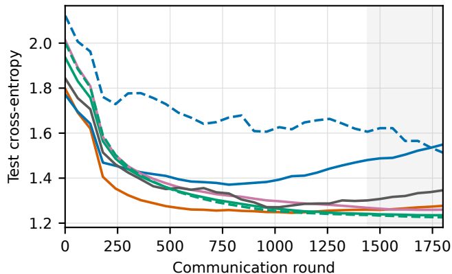
Held-out loss
