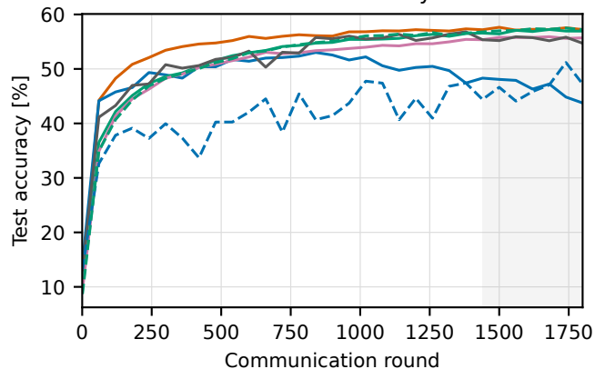
Held-out accuracy
