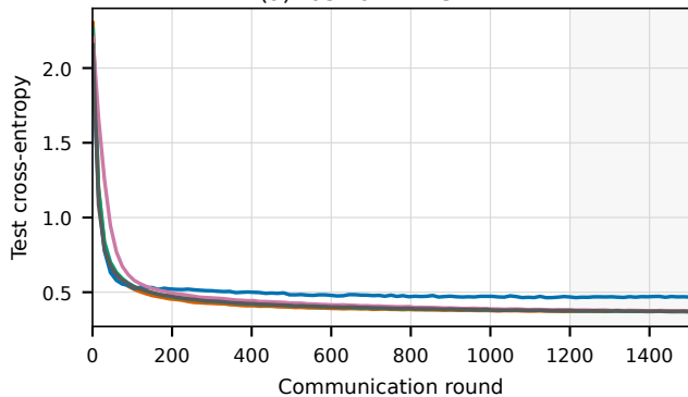
(a) Fashion-MNIST MLP
