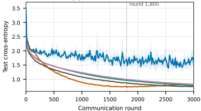
(c) CIFAR-10 ResNet-14
