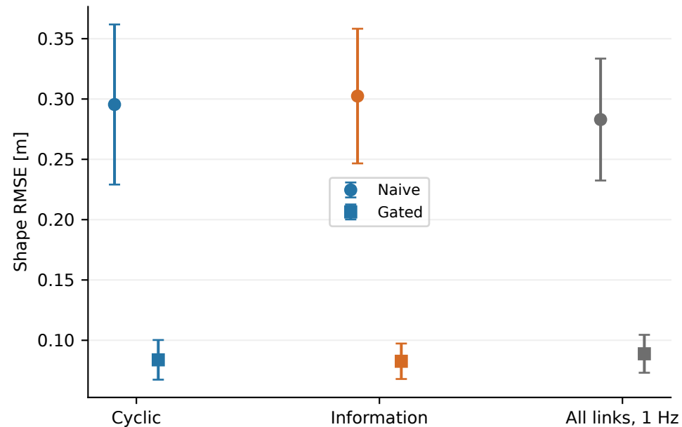
(a) 5% positive outliers, +1 to +3 m
