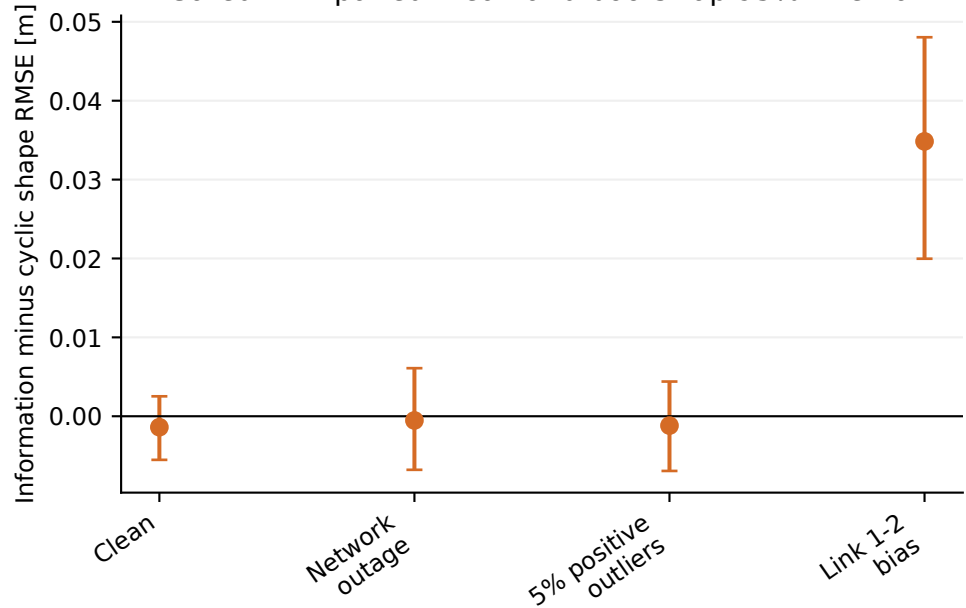
Gated EKF: paired mean and bootstrap 95% interval
