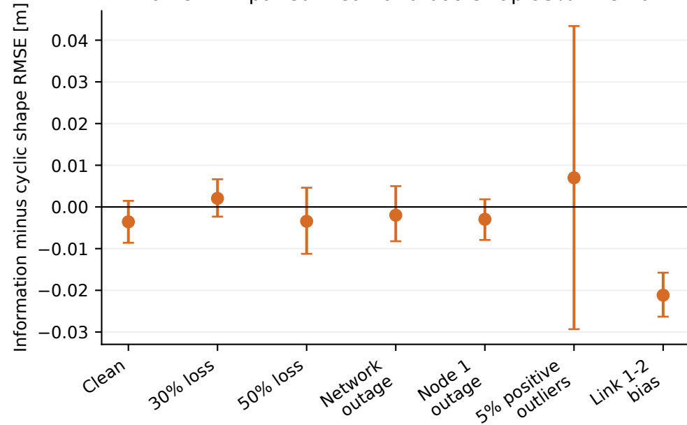
Naive EKF: paired mean and bootstrap 95% interval
