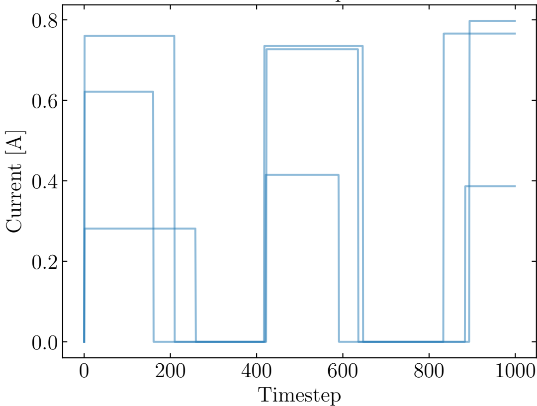
Pulse current profiles
