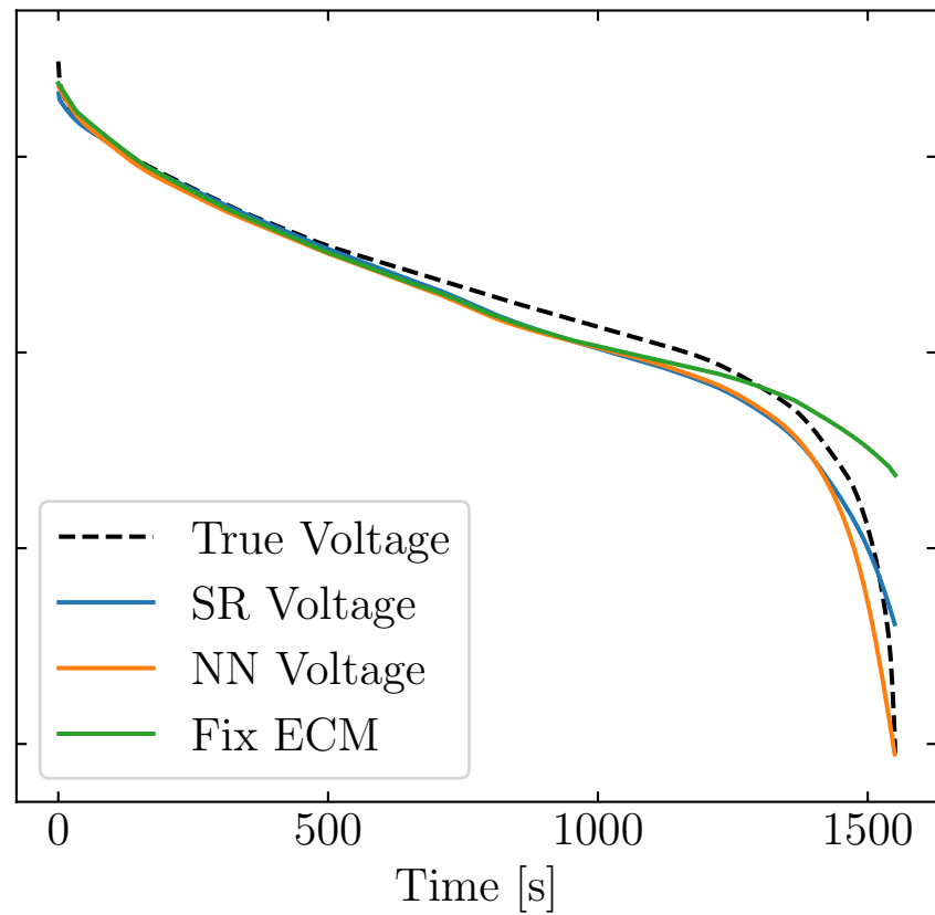
C-rate: 2
