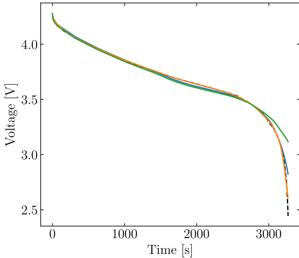
C-rate: 1
