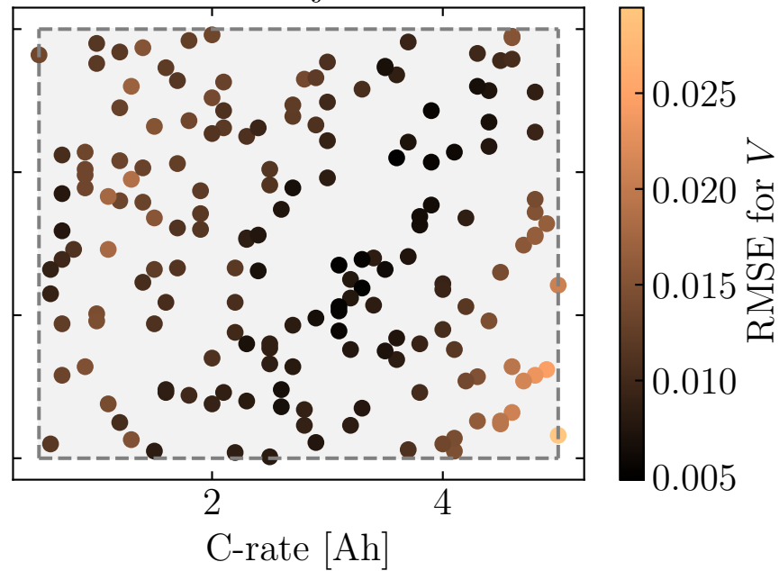
Train Trajectories
