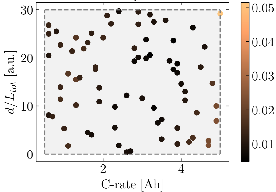
Test Trajectories
