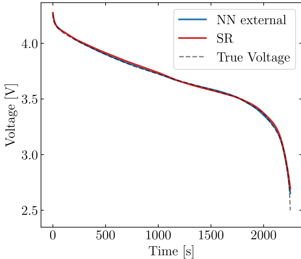
C-rate: 1.5
