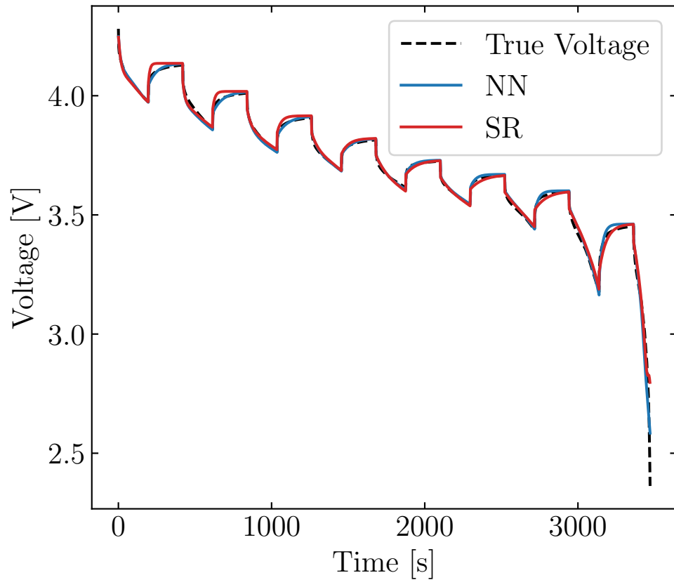
Pulse with max C-rate: 2.0
