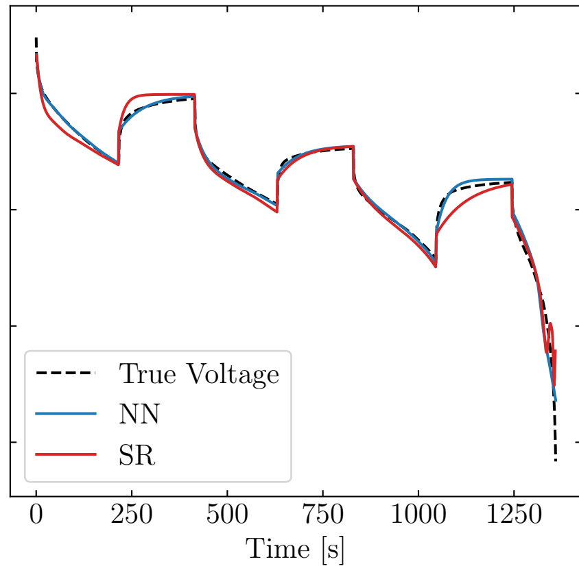
Pulse with max C-rate: 4.0
