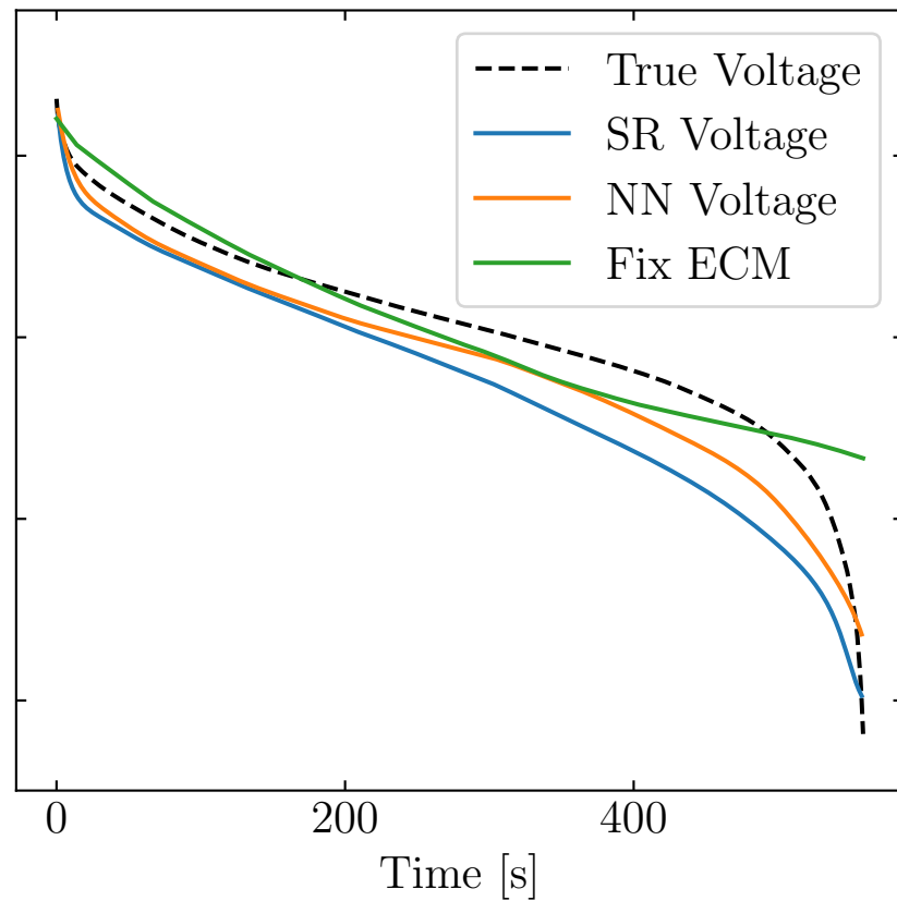
C-rate: 5.0
