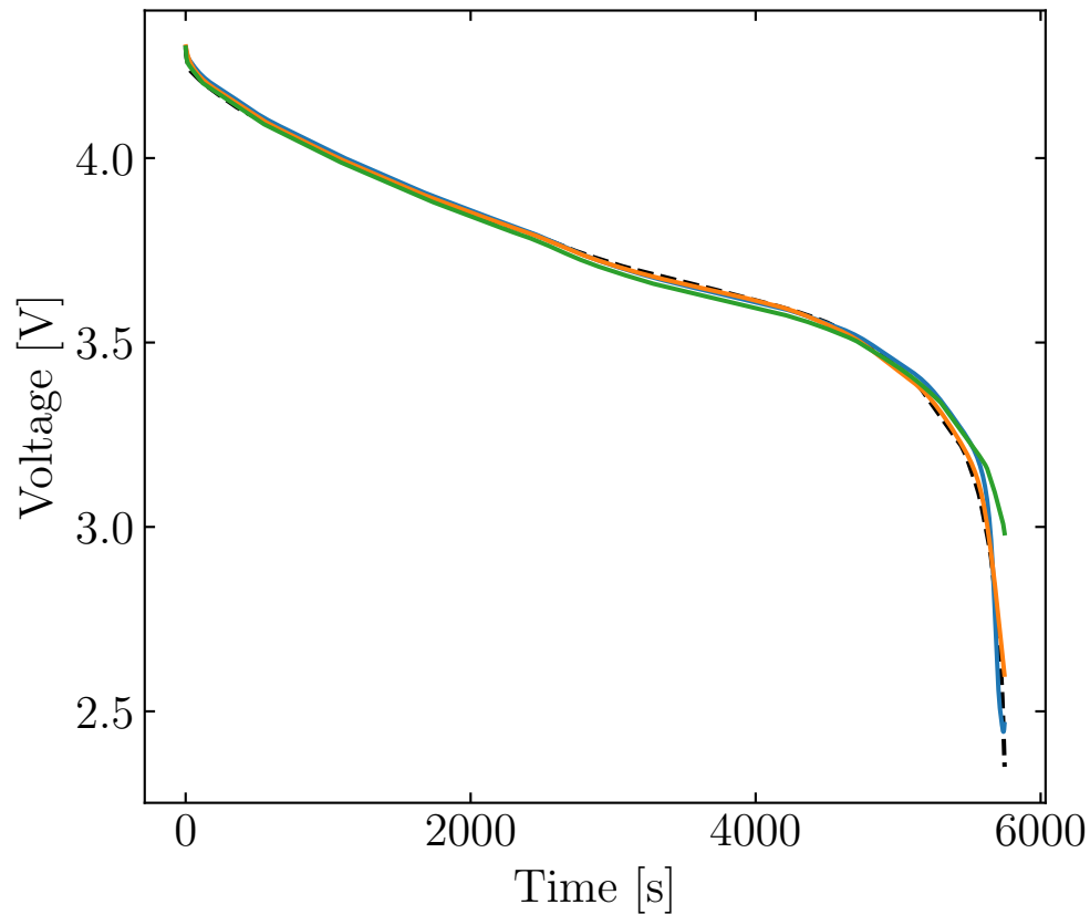
C-rate: 0.6
