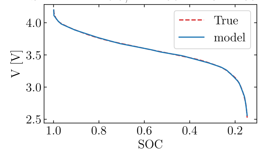
S2 Test: I=15.9, u=-2.961 — C1=188 F
