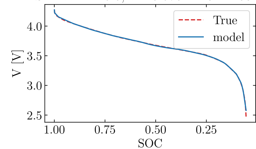
S2 Test: I=6.0, u=-3.076 — C1=188 F
