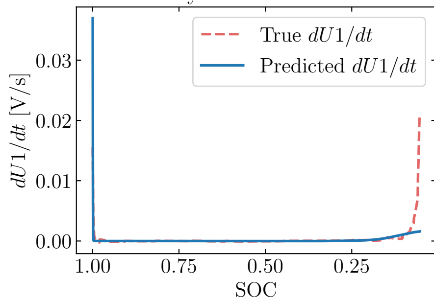
Inferred dynamics with C1=162F
