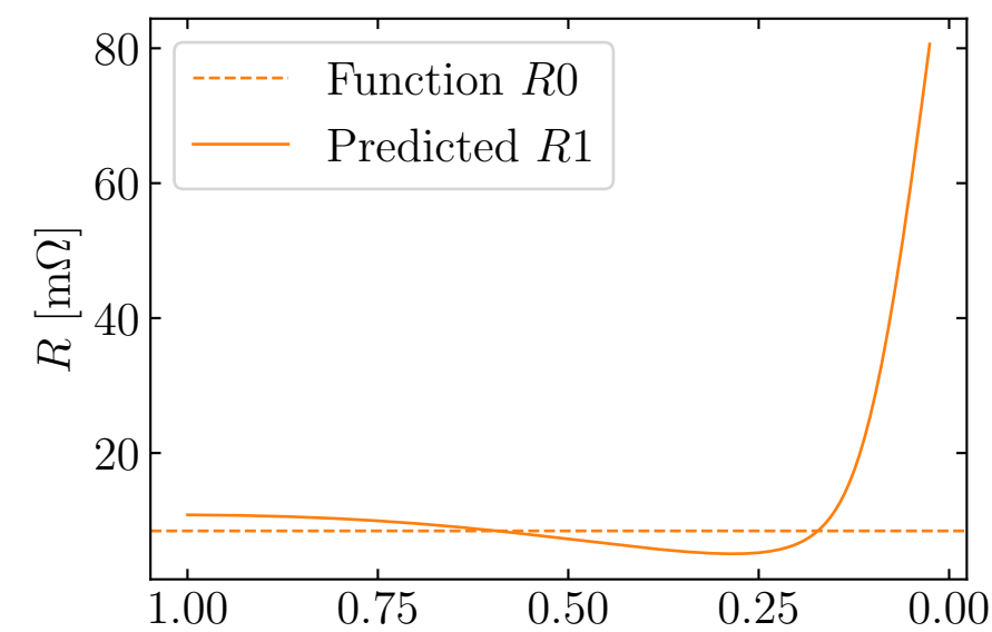
Inferred dynamics with C1=162F
