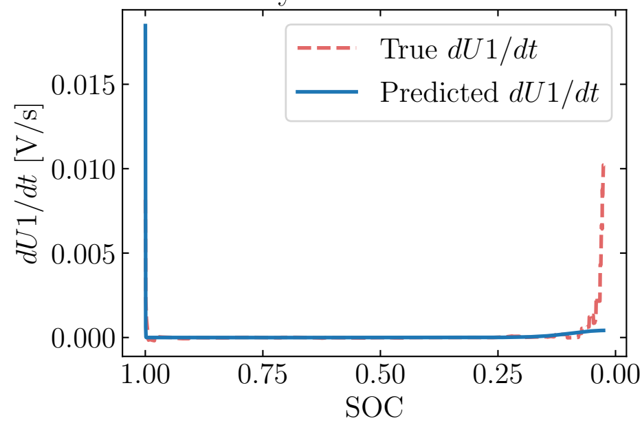
Inferred dynamics with C1=162F
