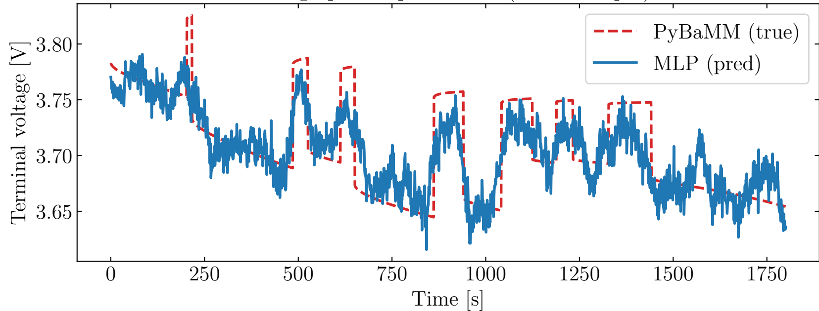
Voltage profile prediction (test example)
