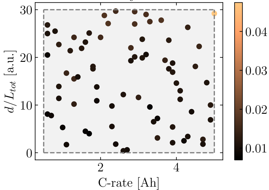
Test Trajectories
