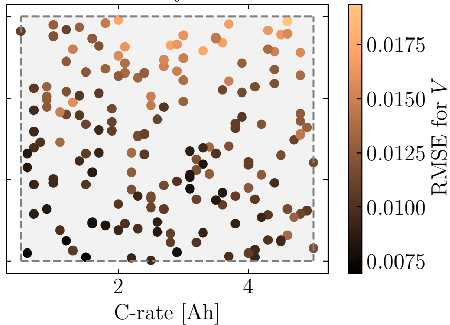
Train Trajectories
