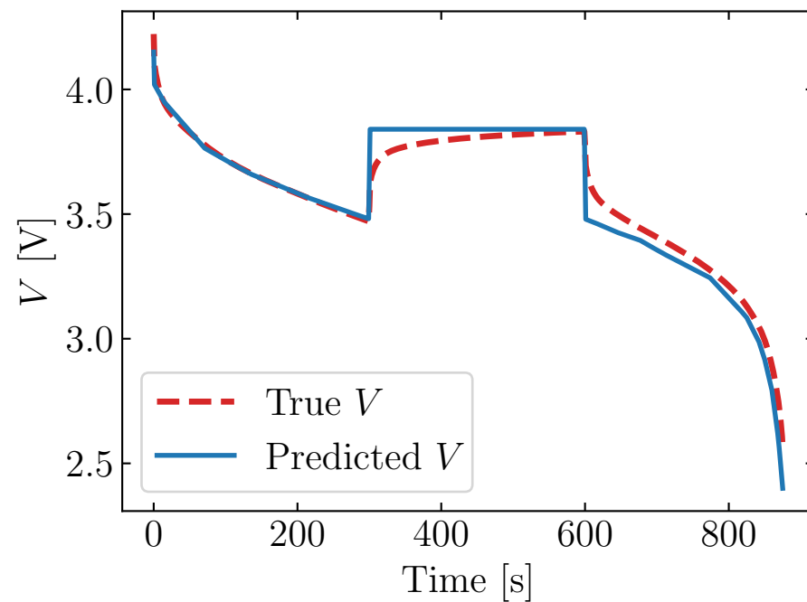
Trajectory 3 c-rate 4.90 Ah
