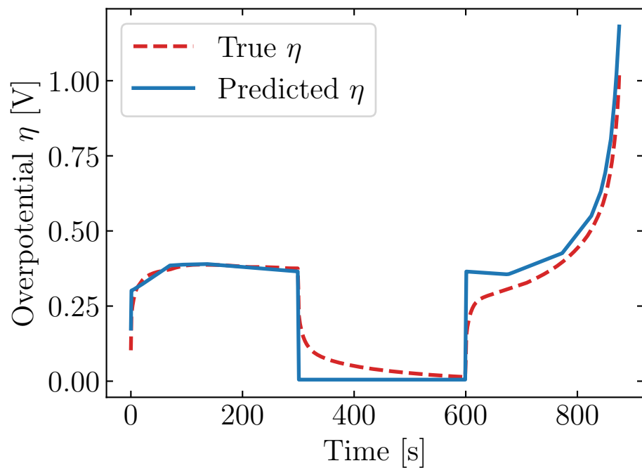
Trajectory 3 c-rate 4.90 Ah
