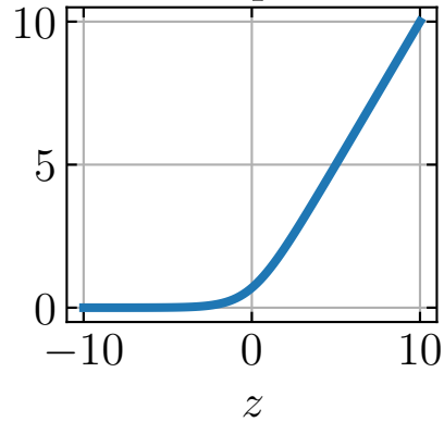
Softplus
