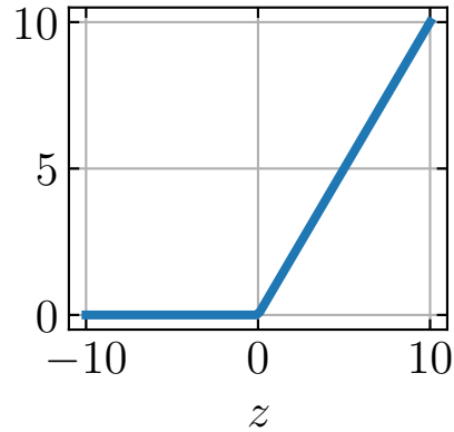
ReLU
