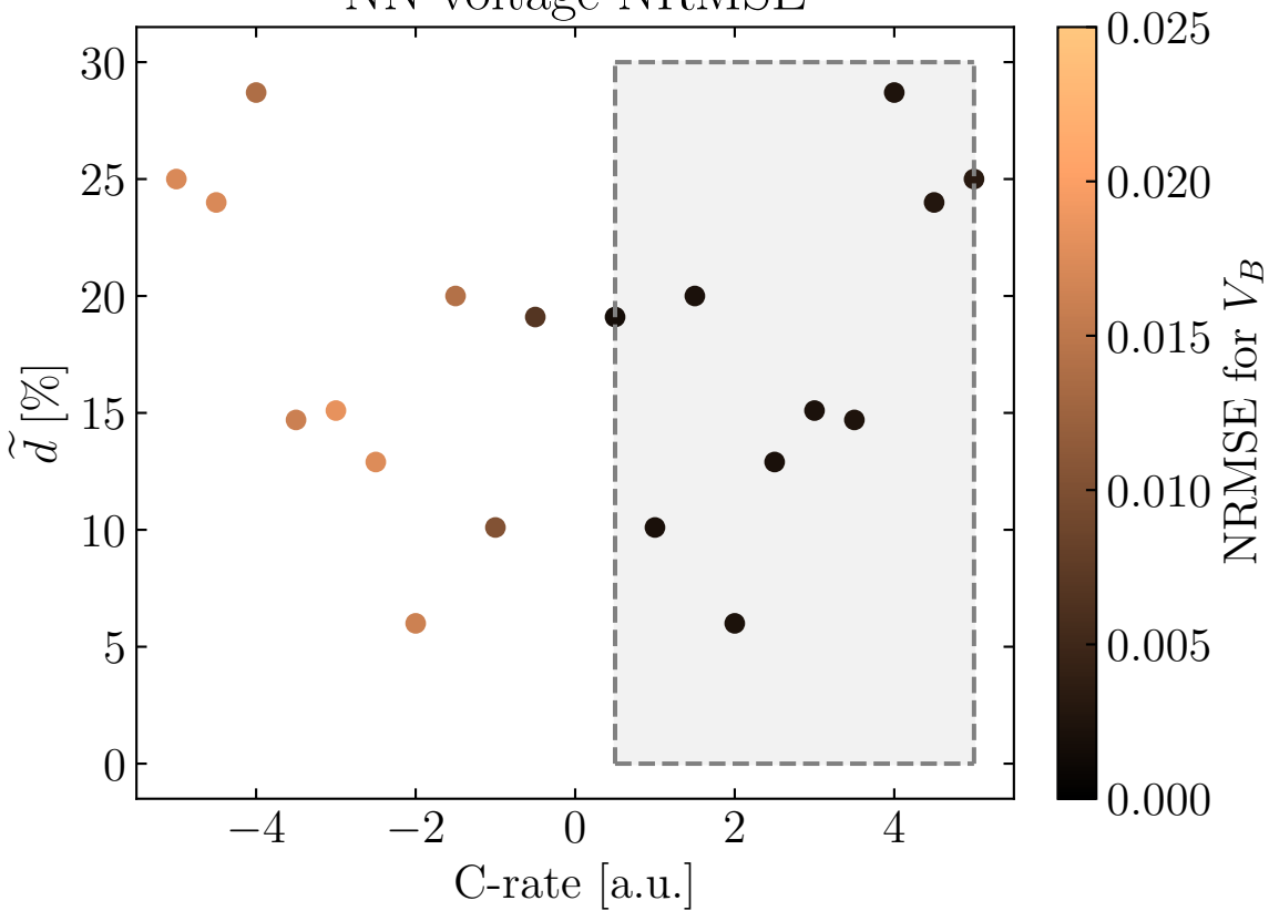
NN voltage NRMSE
