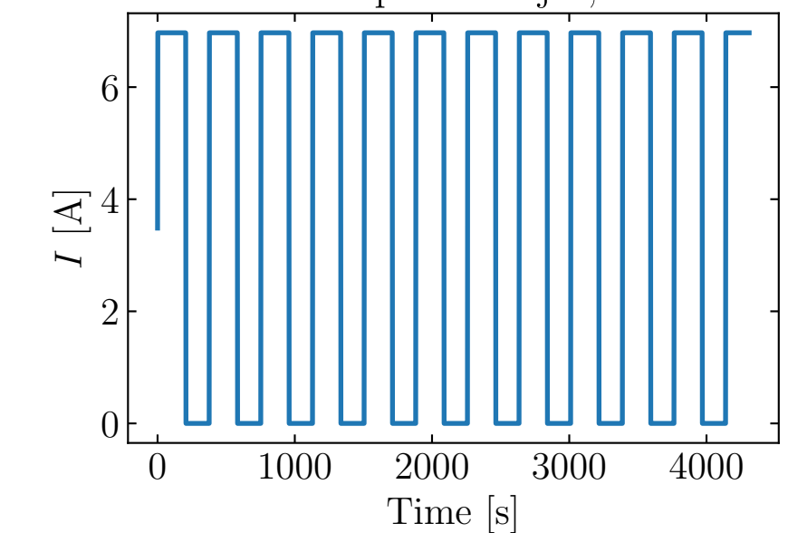
Pulse test: pulse traj 2, u=18.5
