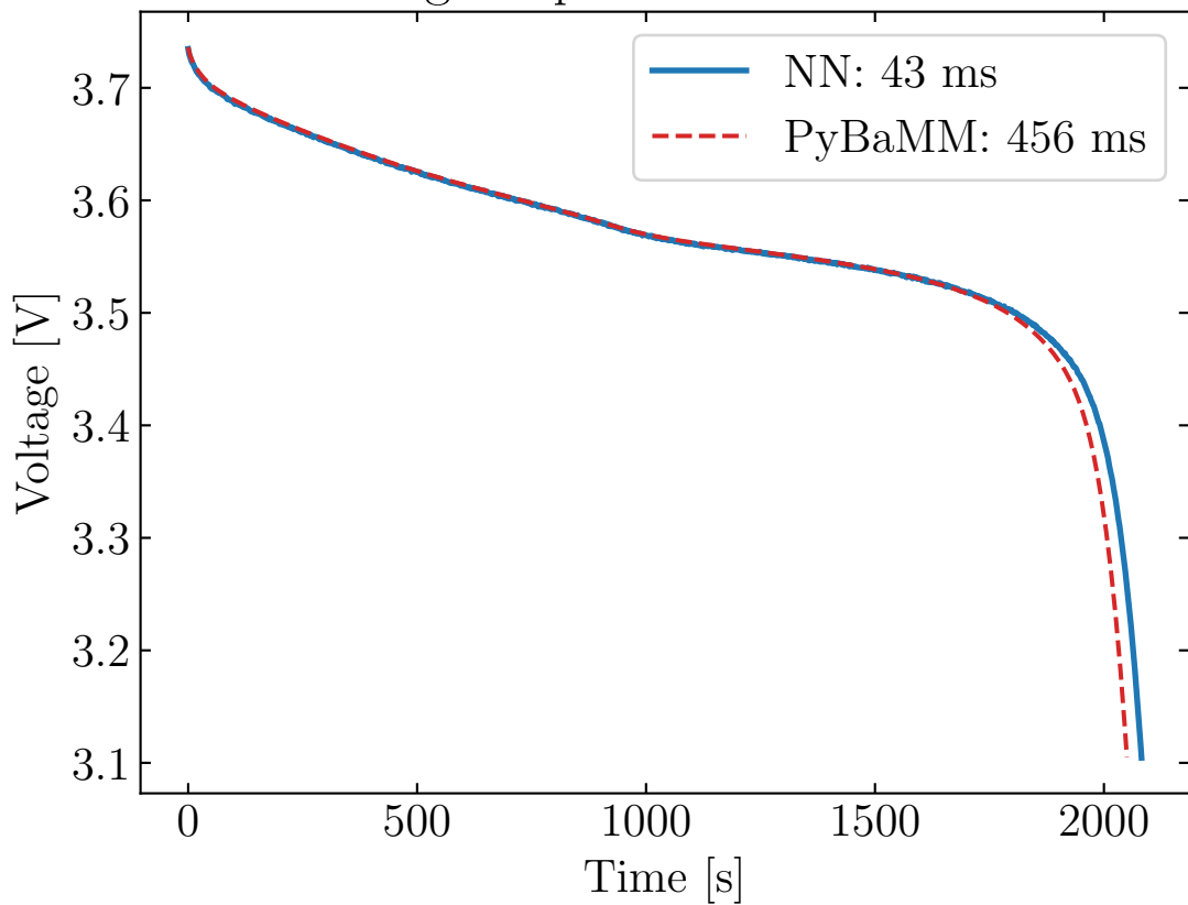
Voltage response for I = 1.18 A
