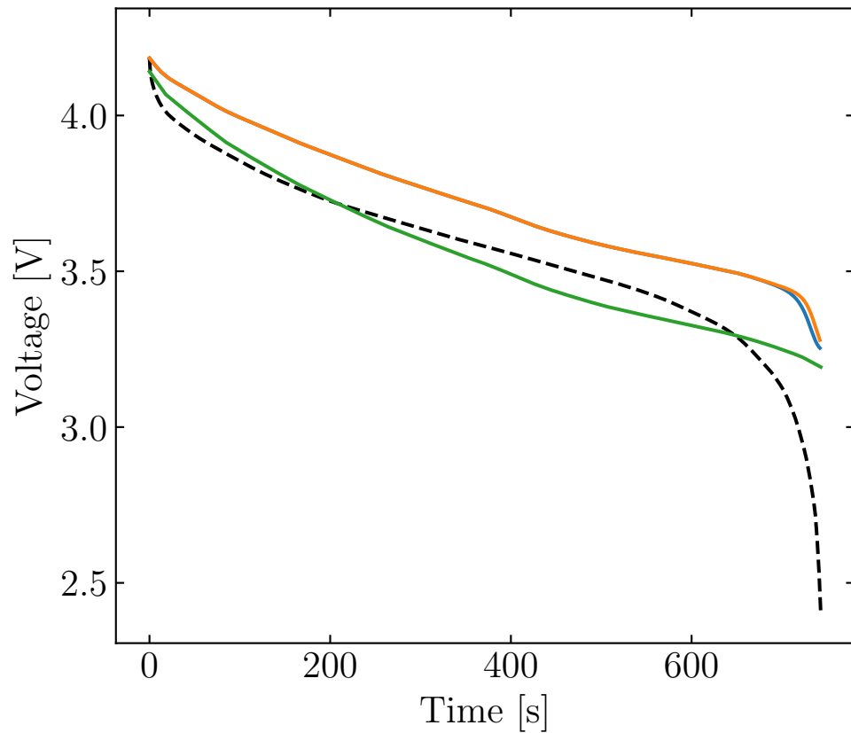
C-rate: 4
