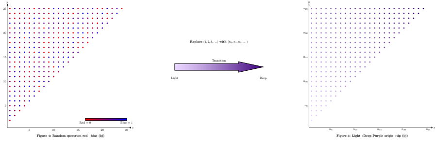
Figure 2.1. Illustration of the (i < j) upper-triangle graphs with a spectrum.
