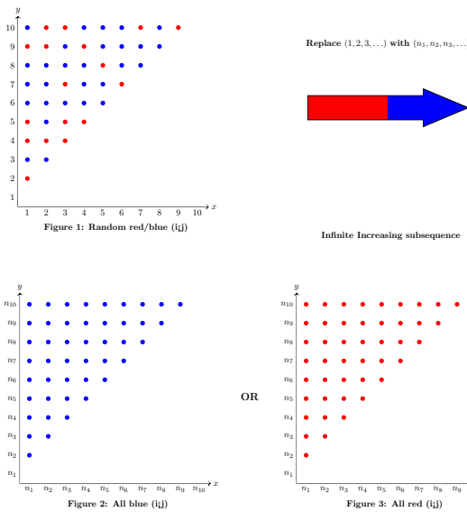
Figure 3.0. Illustration of the (i < j) upper-triangle graphs with 2 colors.
