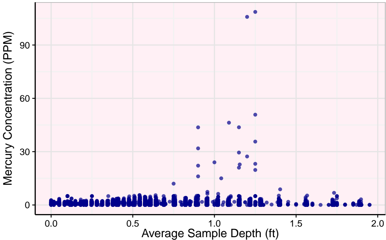
Mercury Concentration vs. Average Depth
