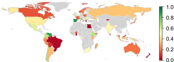
b Beta diversity: Bray-Curtis similarity
