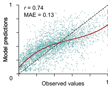
a Training
