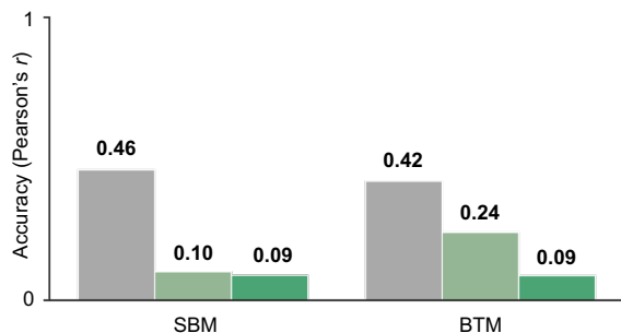
c All site-site pairs within each study and block
