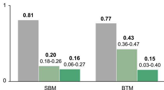
b Beta diversity: Bray-Curtis similarity
