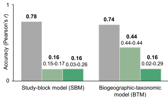
a Alpha diversity: Geometric mean abundance
