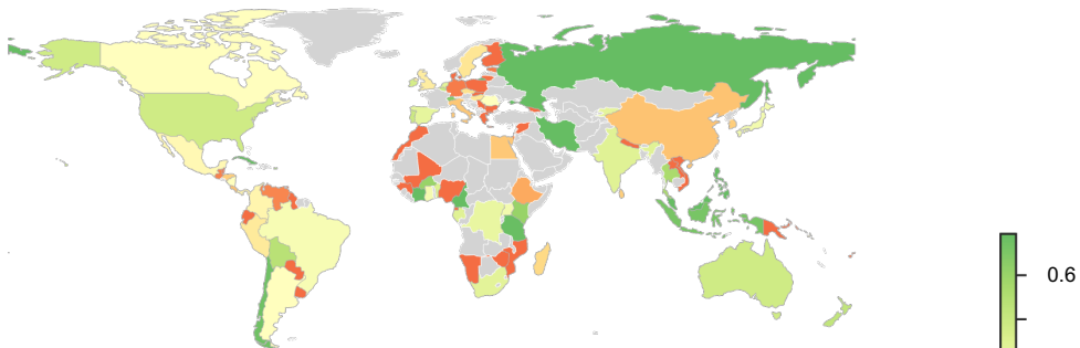
b Beta diversity, standard CV
