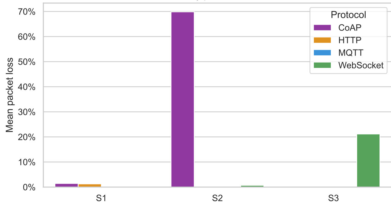
Packet loss by protocol and scenario
