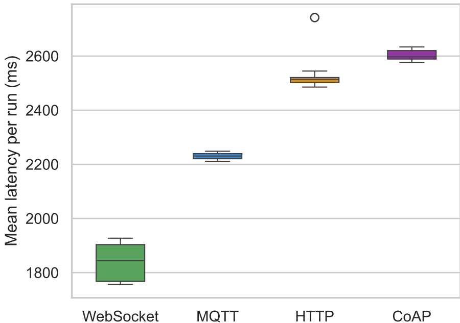
S1 (4 msg/s) — Telemetry latency by protocol (NTP-inflated; relative comparison valid)
