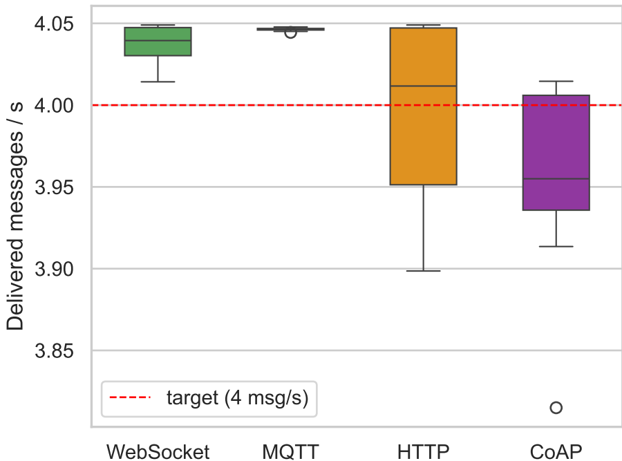
S1 (4 msg/s) — Effective throughput by protocol
