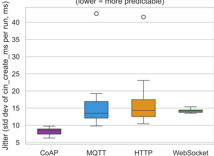
S3 — Command latency jitter by protocol (lower = more predictable)
