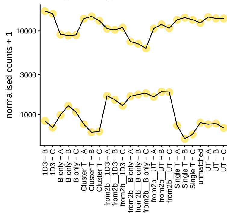
CMV_IE1-17 | profile
