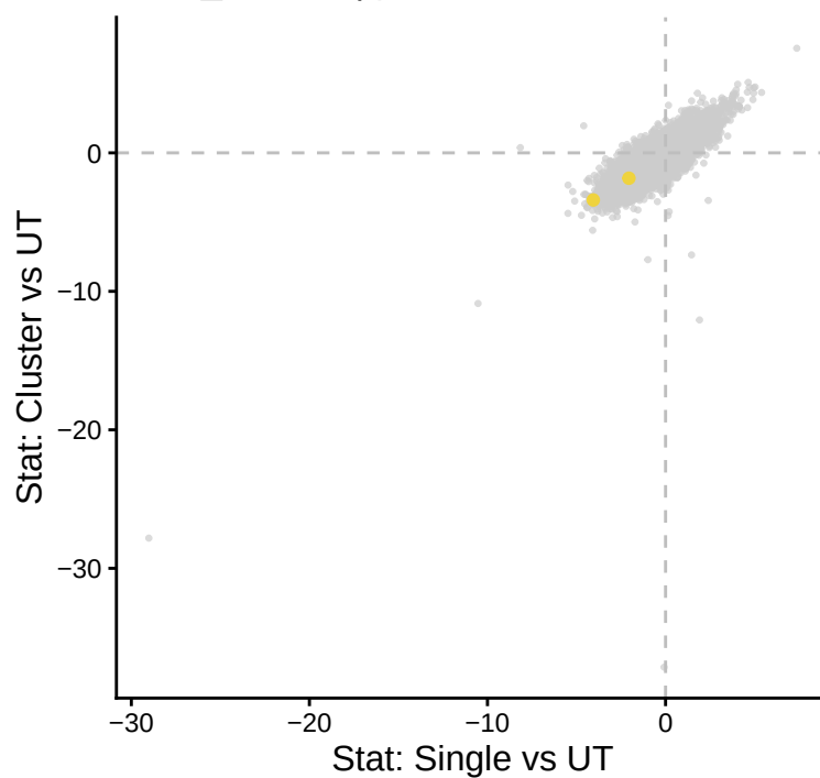
CMV_IE1-17 | pools
