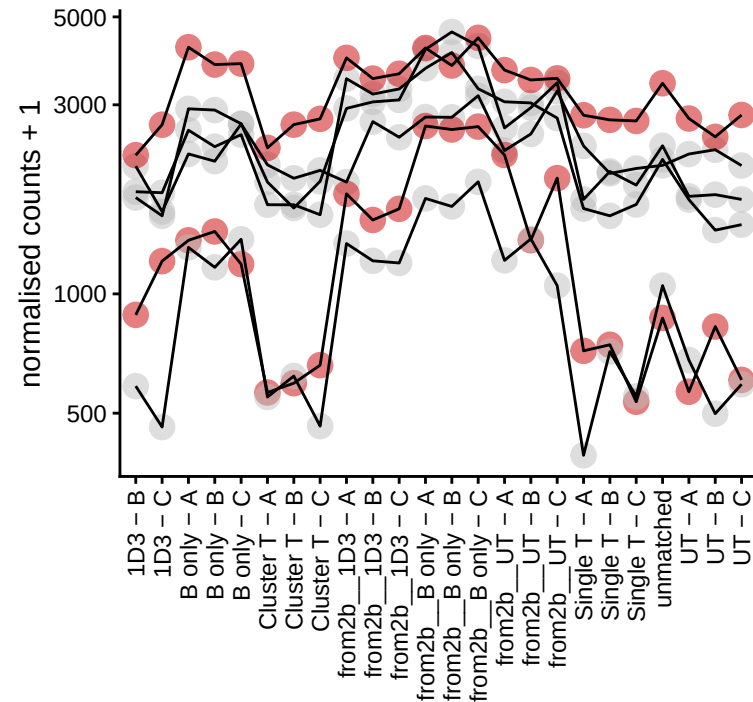
GUCA1A_175fs-1 | profile
