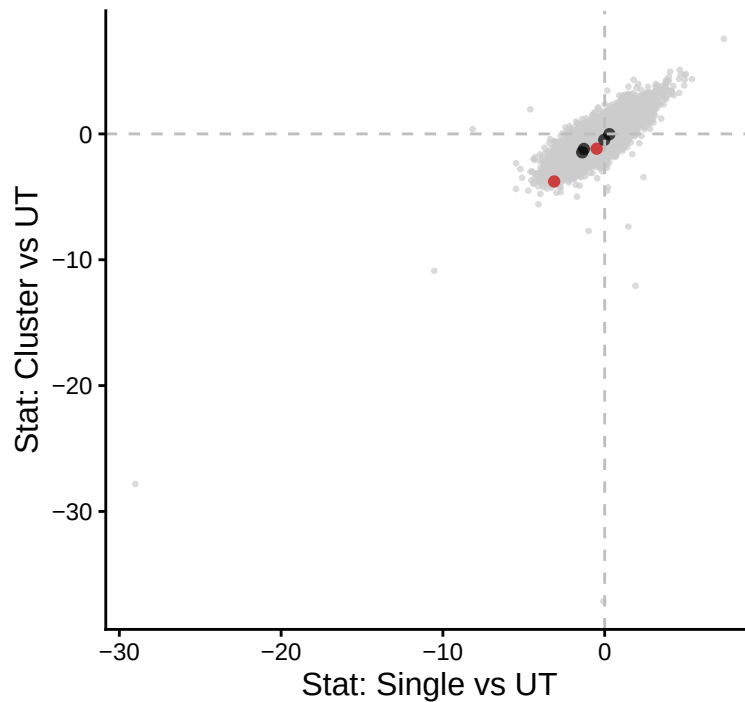
GUCA1A_175fs-1 | pools
