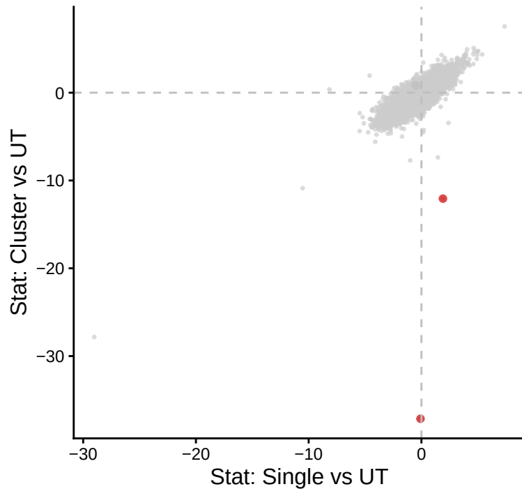
CTR9_T39R | pools
