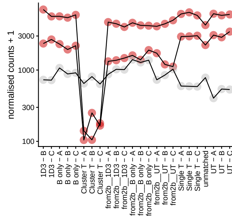
CTR9_T39R | profile
