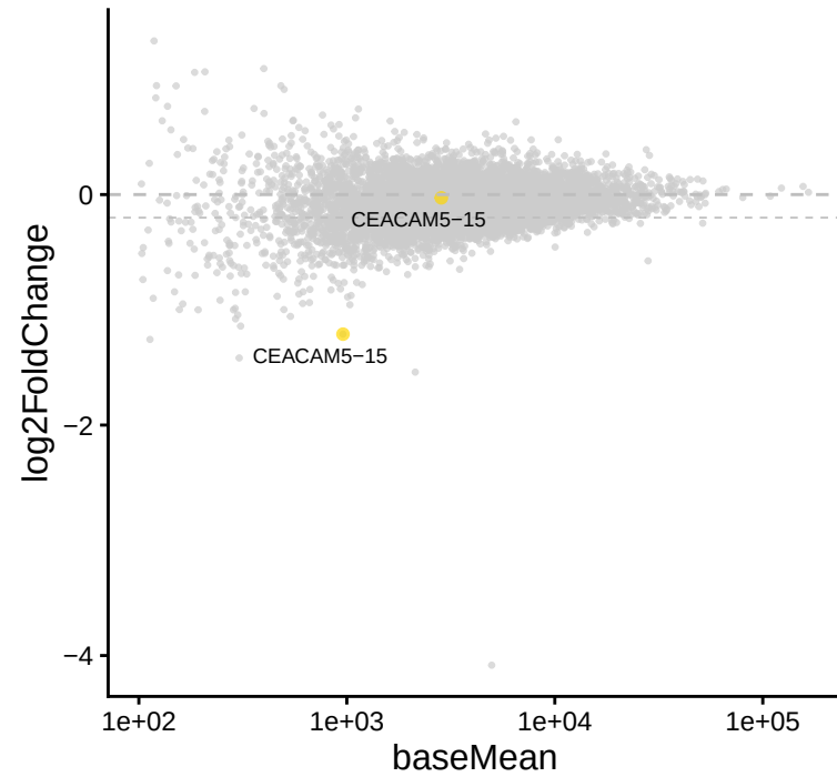
CEACAM5-15 | Single vs UT
