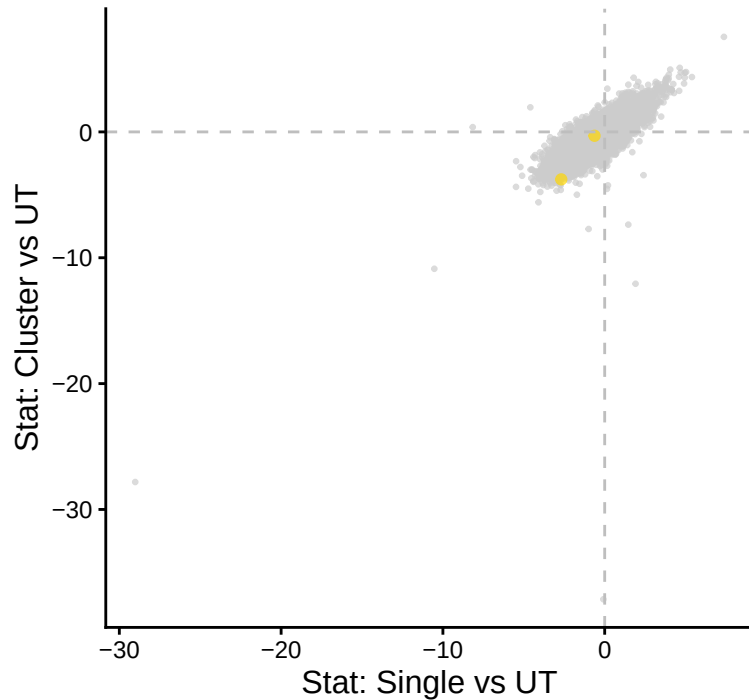
HAGE (DDX43)-8 | pools
