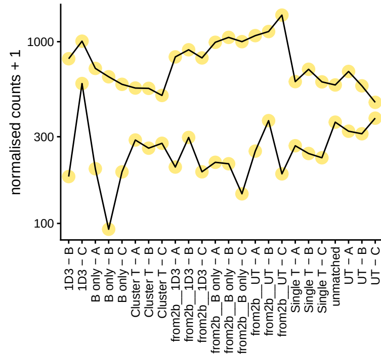
HAGE (DDX43)-8 | profile
