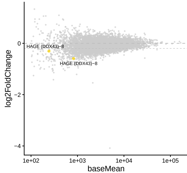
HAGE (DDX43)-8 | Single vs UT
