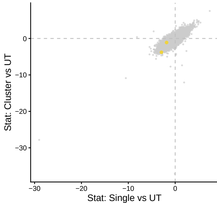
MAGEA12-18 | pools
