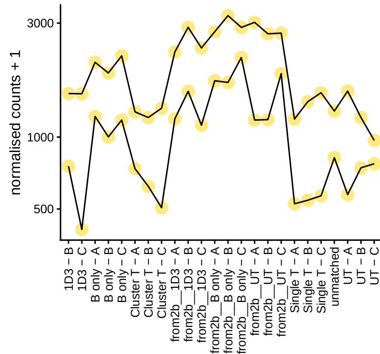
MAGEA12-18 | profile
