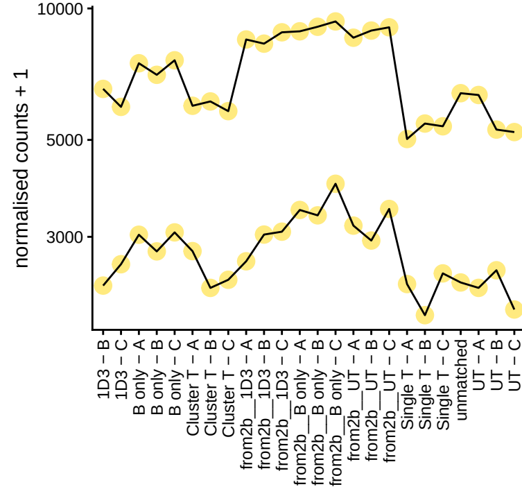
CEACAM5-11 | profile
