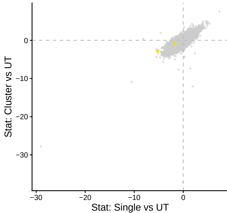
CEACAM5-11 | pools
