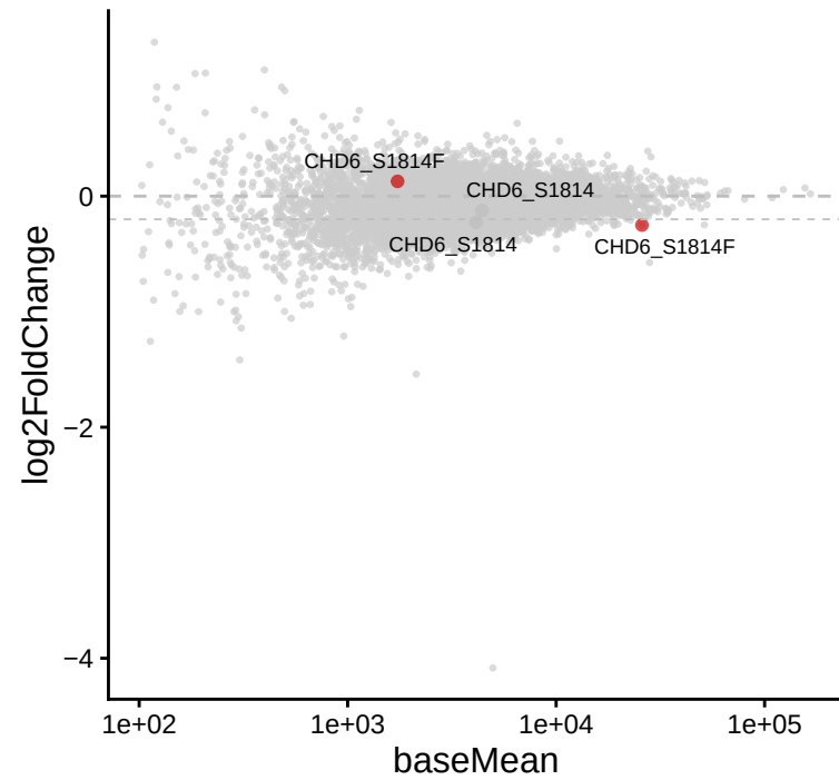
CHD6_S1814F | Single vs UT
