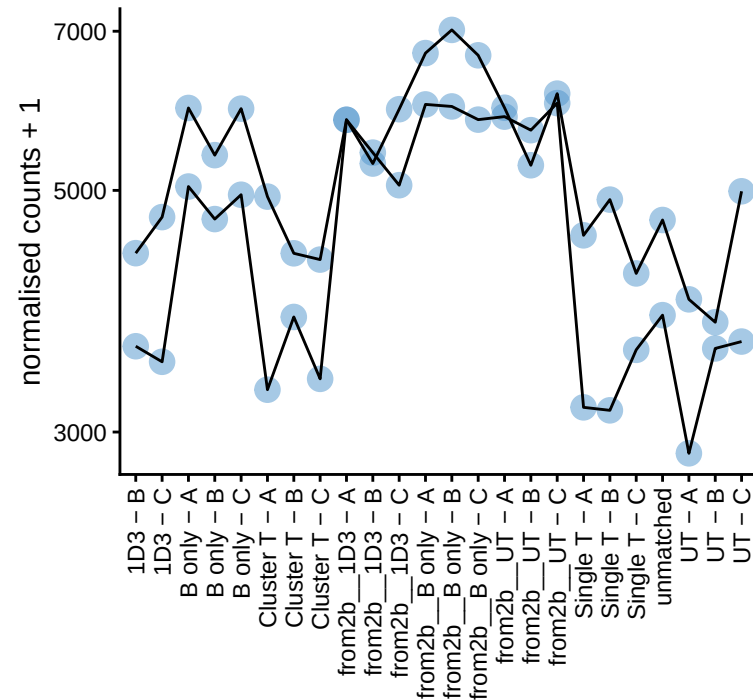
EBV_EBNA4-18 | profile
