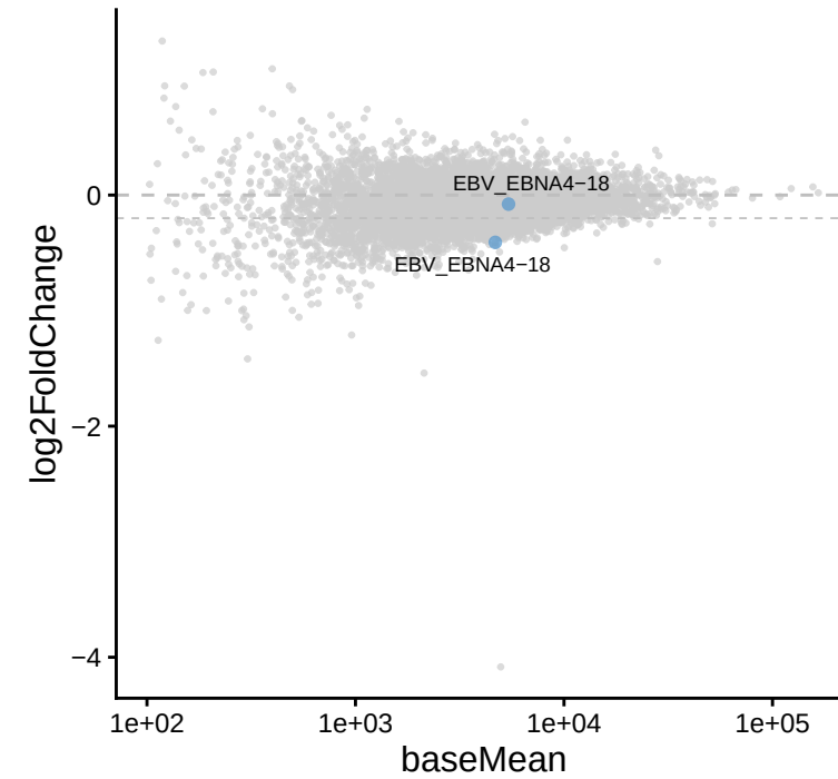
EBV_EBNA4-18 | Single vs UT
