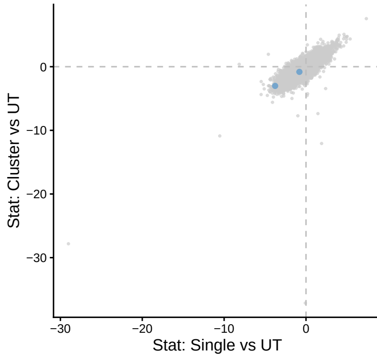
EBV_EBNA4-18 | pools
